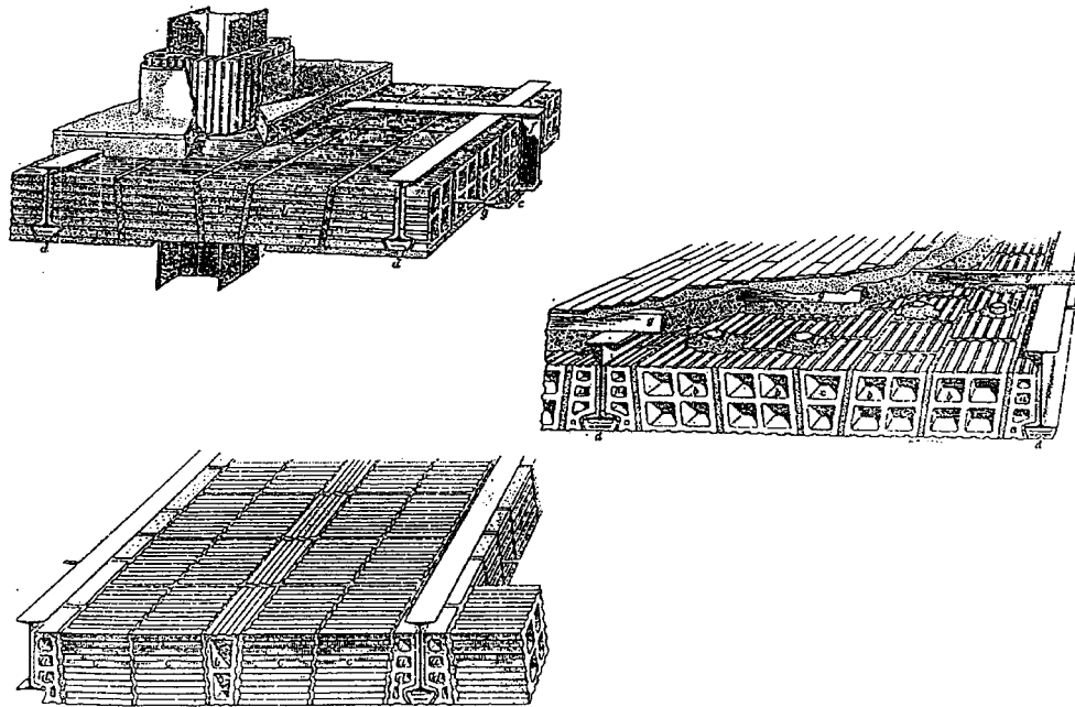
(b) Hollow clay tile flat arch spanning between steel I-beams
