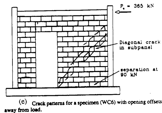
Figure 8-4 Effect of openings on the monotonic lateral-load performance of steel frame-masonry infill tested by Dawe and Seah (1988).
