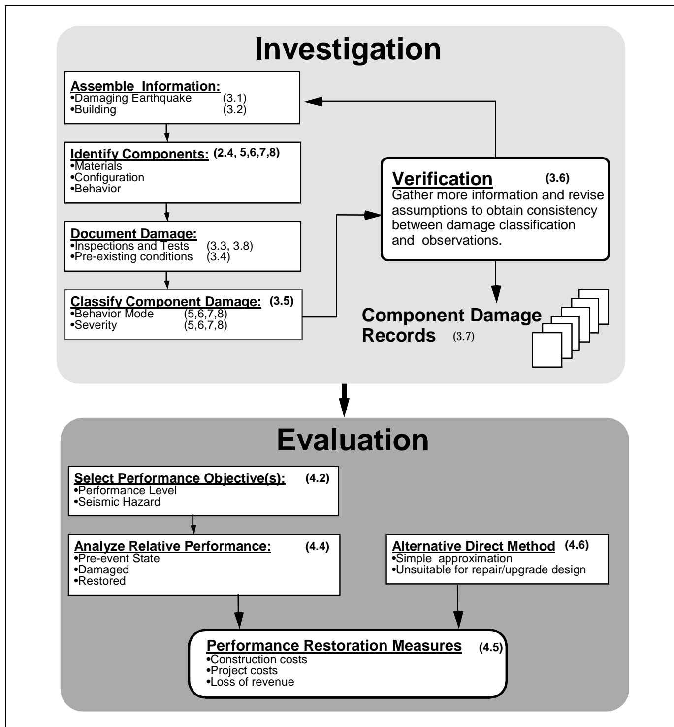
Figure 1-3 Flowchart for the Investigation and Evaluation of Earthquake Damage to Concrete and Masonry Wall Buildings. (Section numbers are indicated.)
