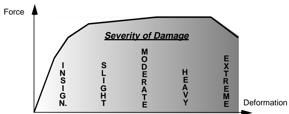
a) High ductility behavior
