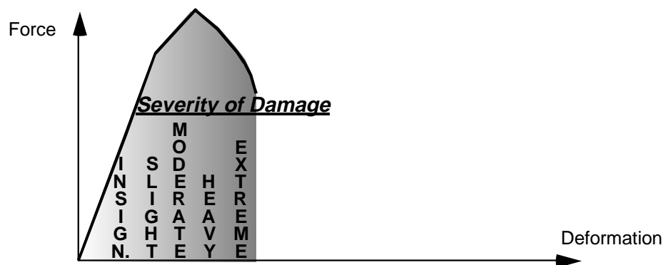
c) Low ductility behavior
