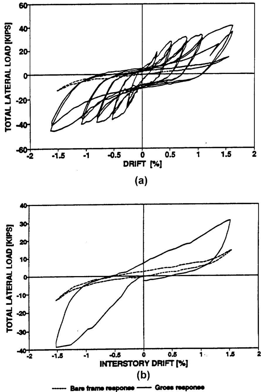
Figure 8-3 Specimen tested by Mander et al. (1993a). Steel frame-clay brick masonry infill. Top and seat angles semi-rigid connections used to connect beams to columns. (a) Original specimen. (b) Specimen repaired with 1/2-inch ferrocement overlay and retested.
