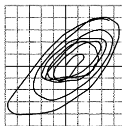
Hysteretic Response
