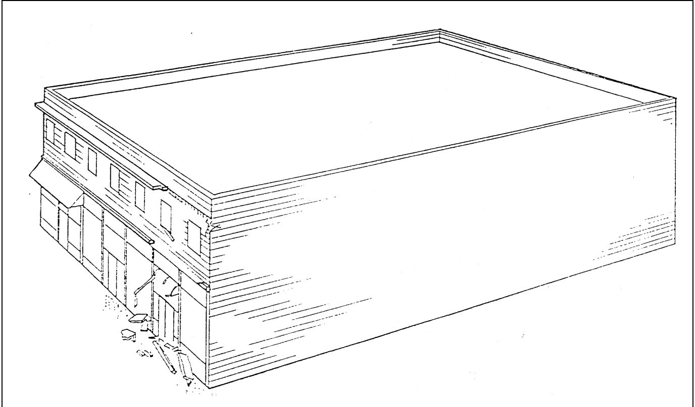
Figure 7-3 Diagram of an Appendage Failure (from Rutherford and Chekene, 1990)
