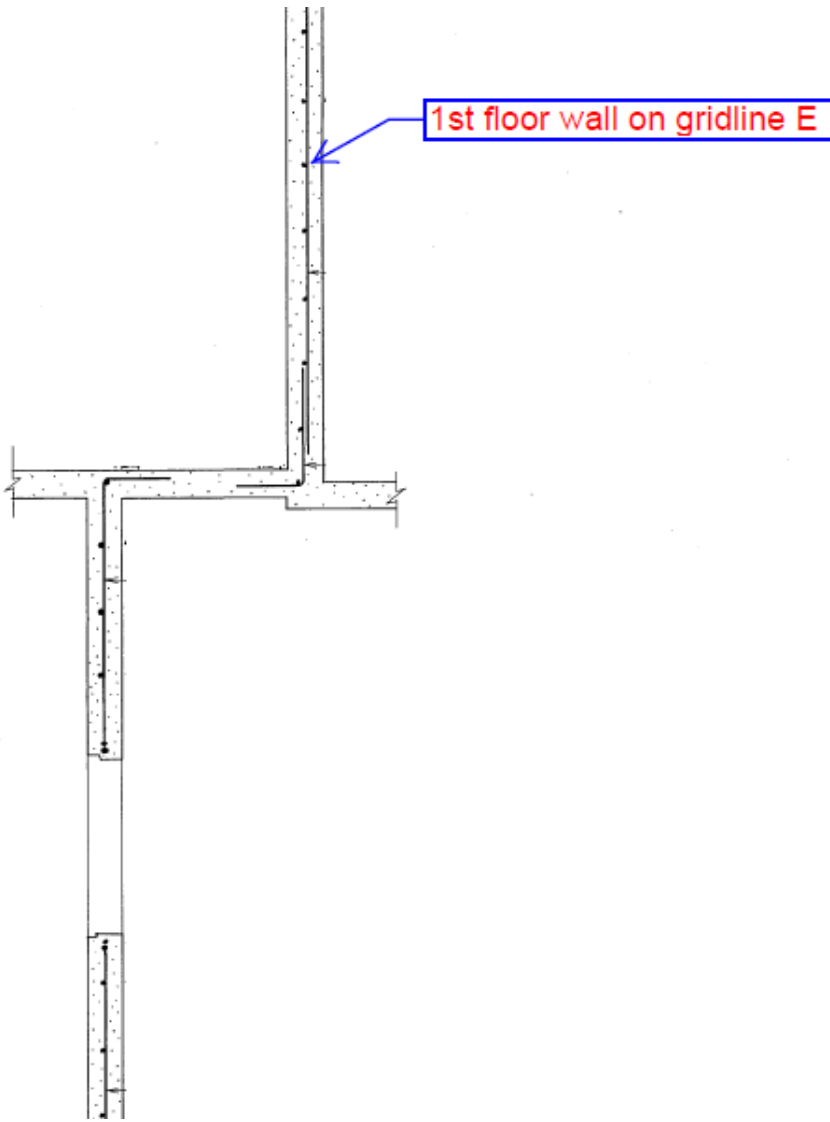
Partial Cross Section from original drawings showing offset of 1 st floor wall from ground floor wall.
