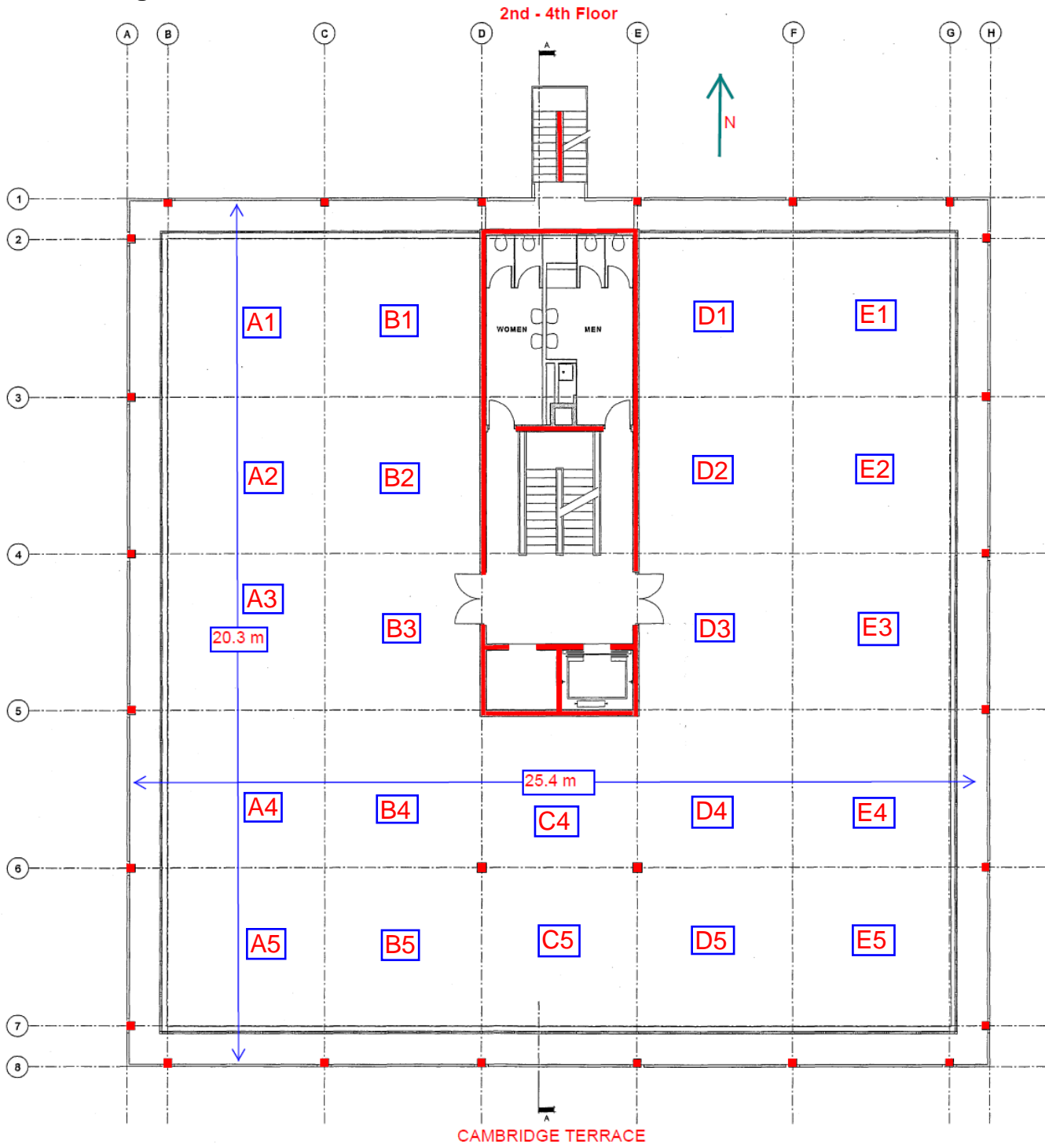
Second, Third & Fourth Floor Plan
