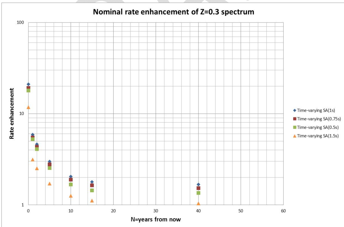
Figure 10 Rate enhancement of Z=0.3 spectral accelerations with respect to the nominal annual exceedance rate of 1/500 for the Ultimate Limit State Restricted to range of intended applicability).
