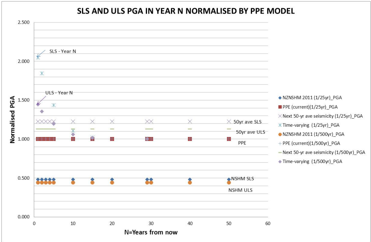
Figure 9 SLS and ULS pgas for liquefaction analyses as in Figure 8 normalised by the PPE model that gives the constant seismicity rates that are reached by about 20 years or sooner from now.
