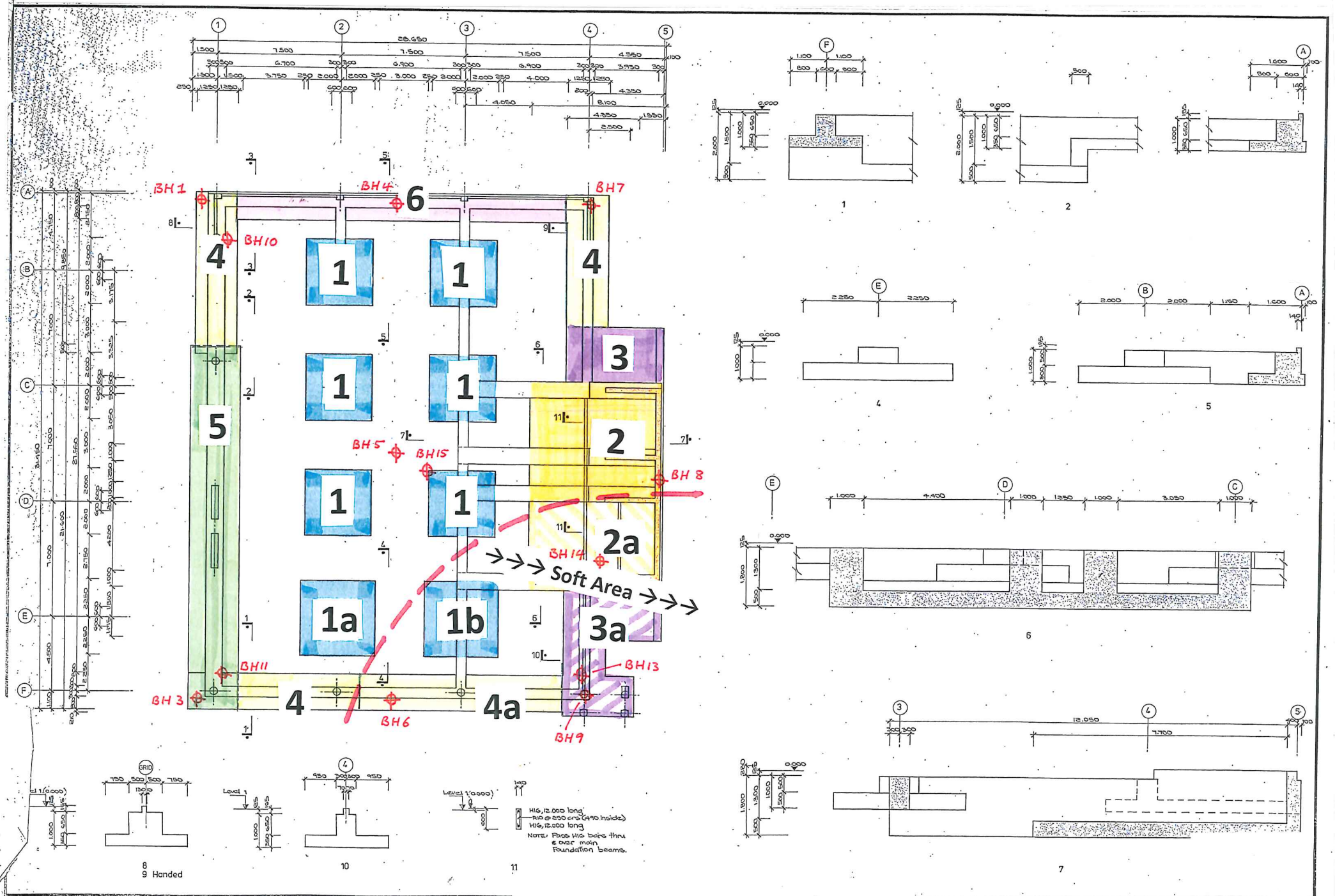
Figure 1: Foundation Types
