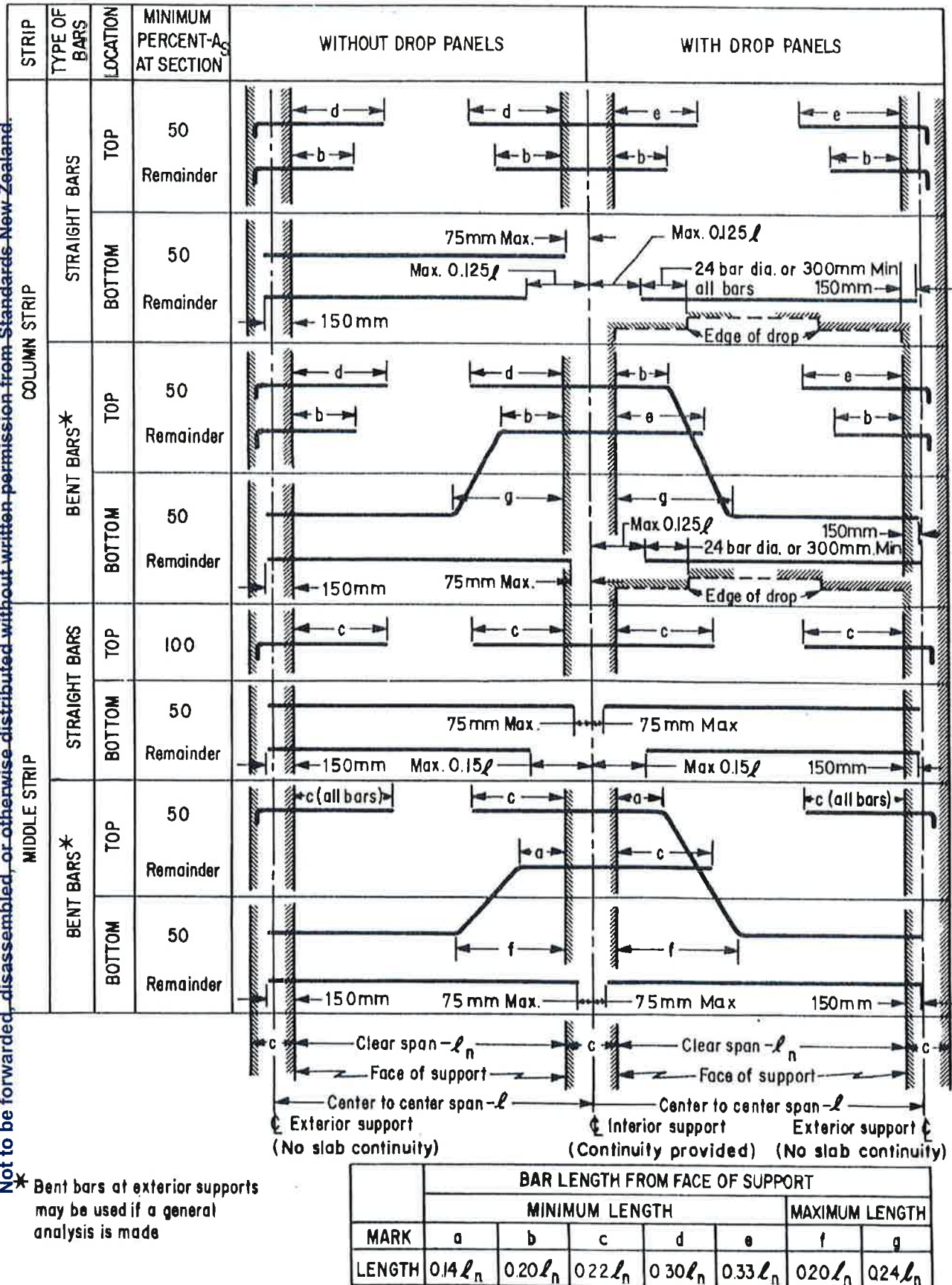
Fig. 11.3 MINIMUM BEND POINT LOCATIONS AND EXTENSIONS FOR REINFORCEMENT IN SLABS WITHOUT BEAMS (see 5.3.25.1 for reinforcement extension into supports)
