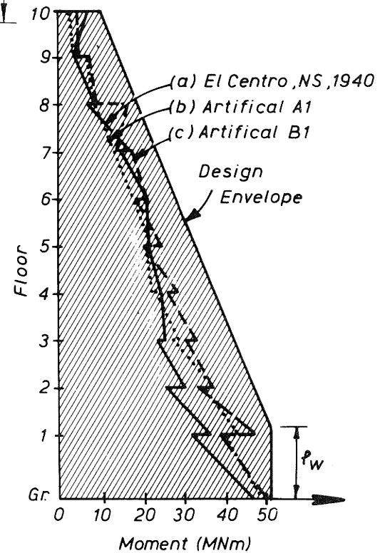
Fig. 19 - Bending Moment Envelopes for Coupled Shear Walls (a) Envelope Used in Design (b) Envelopes Observed in a Theoretical Study (15).
