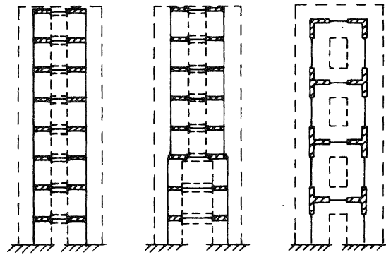
WIDE COLUMN FRAME (a)
