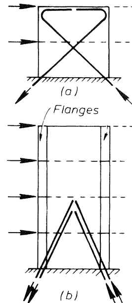
Fig. 26 - Suggestions for the Arrangement of Diagonal Reinforcement to Control Sliding Displacement at the Base.
